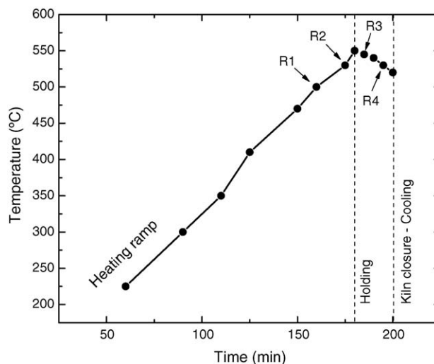
Fig. 1. Relation between temperatures and time during samples extraction from the traditional kiln. Samples were extracted in the temperature range 500–550 °C, when the traditional kiln reached the maximum of the heating ramp.
